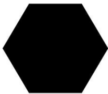
육각형 (Hexagon)
