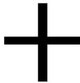
더하기 (Addition)
